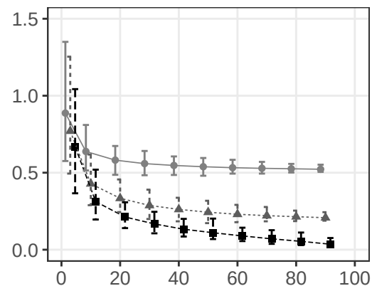
Number of Negative ICCs
